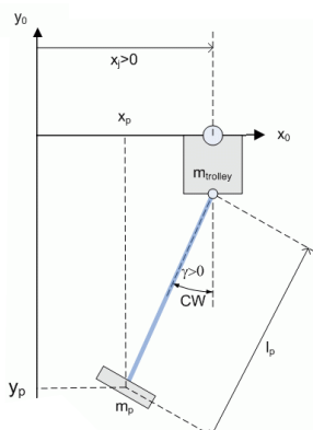
Figure 1. Linear gantry challenge teaches how to minimize payload swings as the trolley move across the jib.
